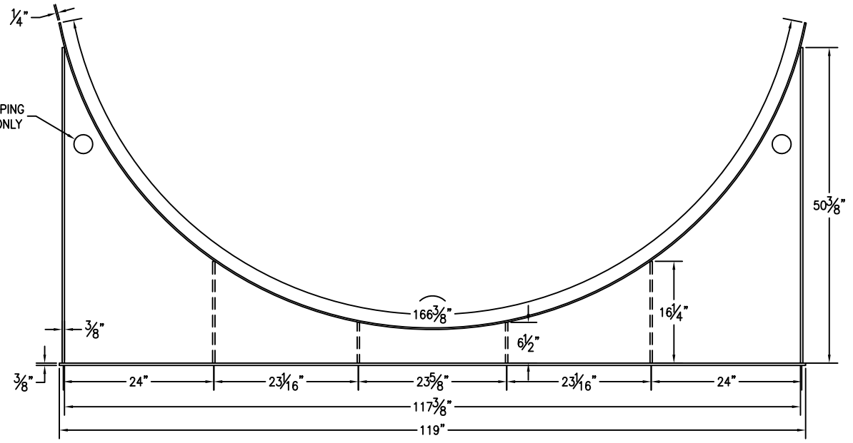
BASE PLATE ANCHOR HOLE DETAIL
