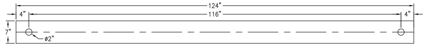
BASE PLATE ANCHOR HOLE DETAIL
