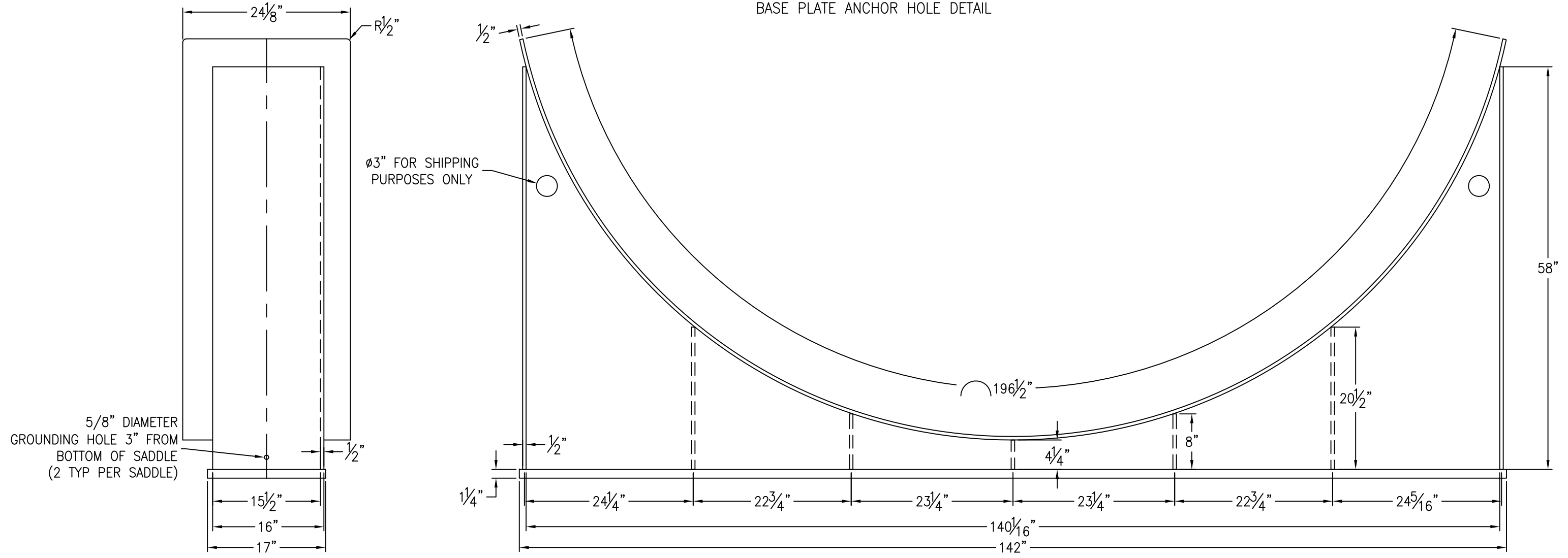
BASE PLATE ANCHOR HOLE DETAIL
