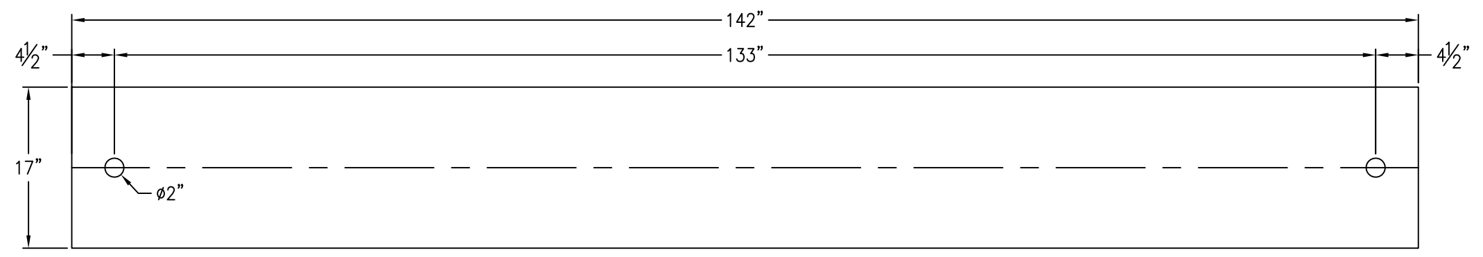
BASE PLATE ANCHOR HOLE DETAIL
