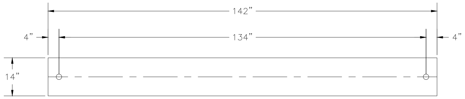
BASE PLATE ANCHOR HOLE DETAIL
