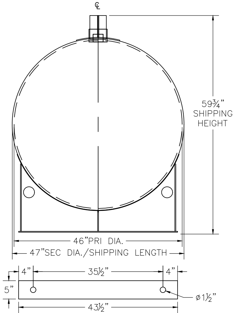
BASE PLATE ANCHOR HOLE DETAIL
